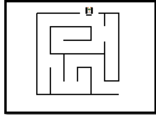
Maze Solver
